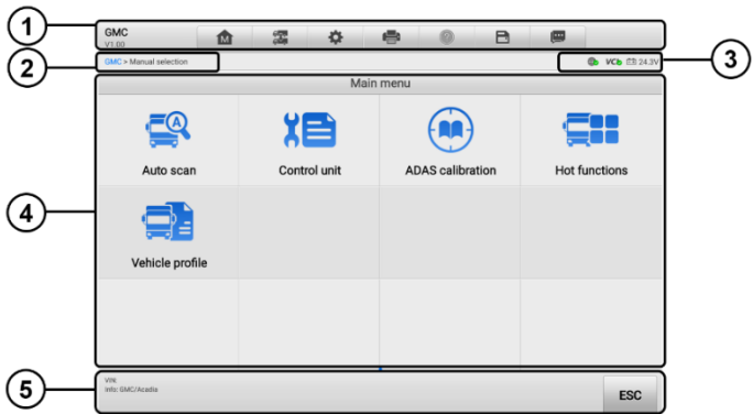
Figure 4-6 Main Menu Screen
