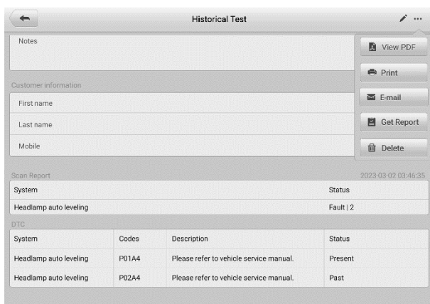
Figure 4-20 Historical Test Screen
