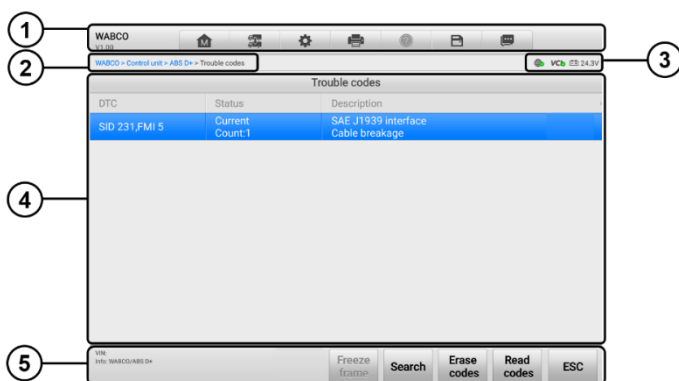
Figure 4-11 Read Codes Screen
