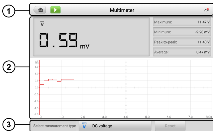
Figure 7-1 Multimeter Screen
