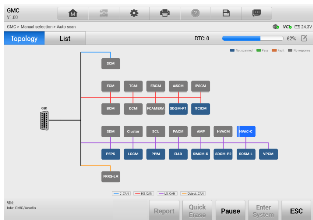
Figure 4-8 Topology Screen
