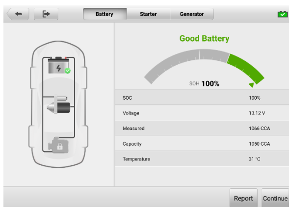
Figure 6-5 Battery Test Results Screen
