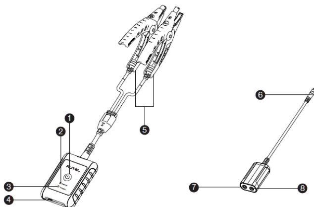
Figure 2-5 MaxiBAS B200 Device
