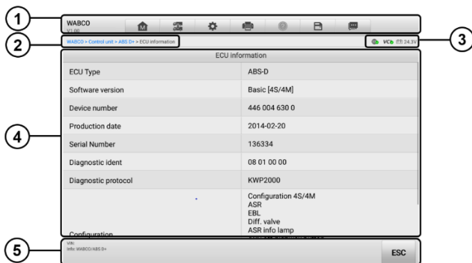
Figure 4-10 ECU Information Screen
