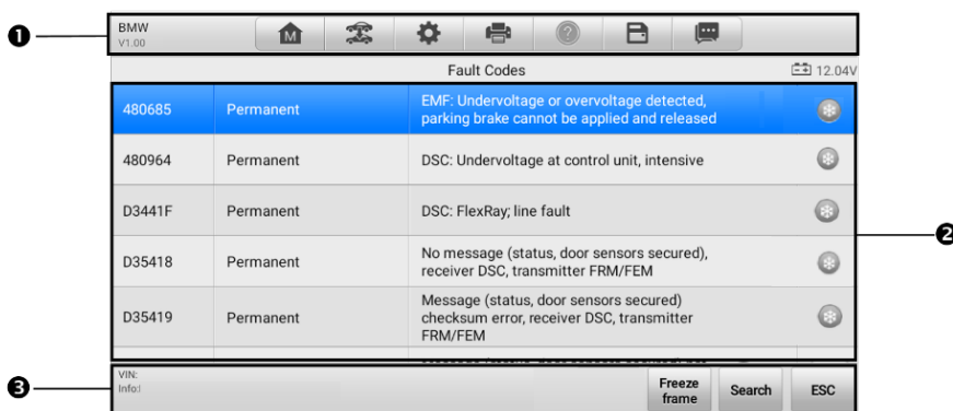
Figure 4-12 Read Codes Screen
