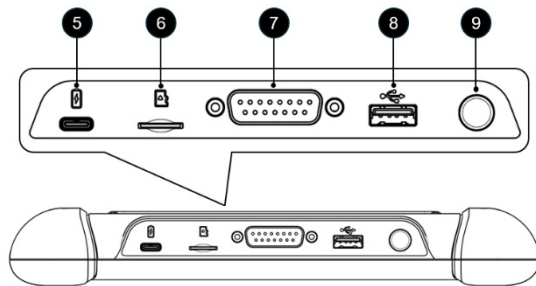
Figure 2-2 Tablet Top View
