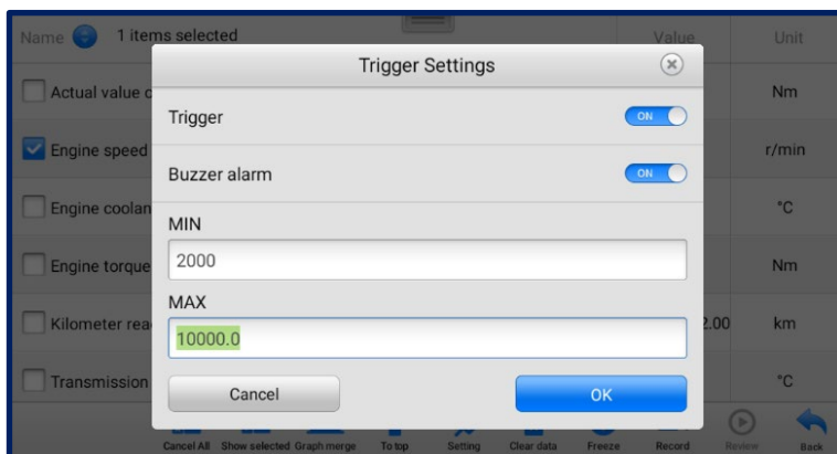
Figure 4-17 Trigger Setting Screen
